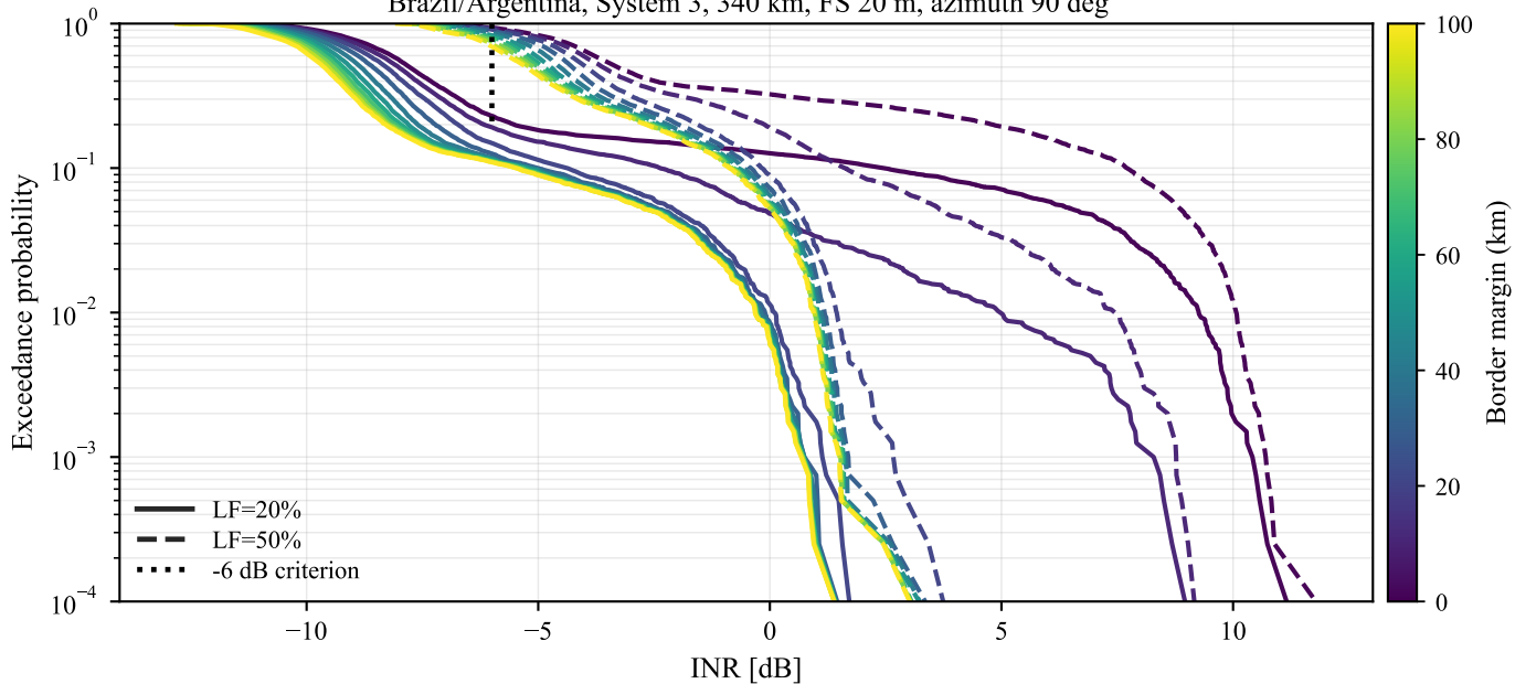
Brazil/Argentina, System 3, 340 km, FS 20 m, azimuth 90 deg
